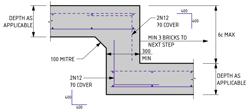
FOOTING STEP
